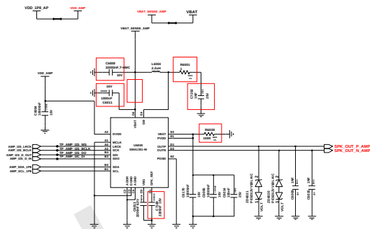
Audio amp
