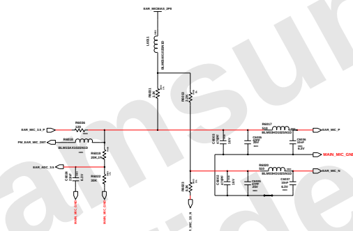
EAR MIC
