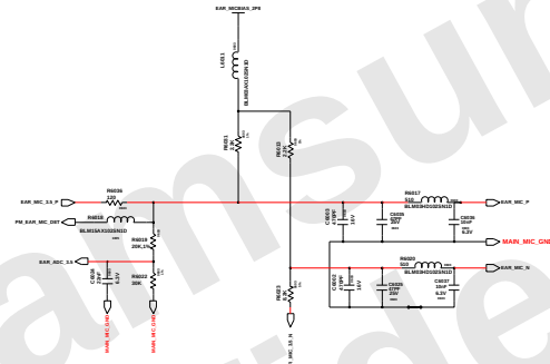
EAR MIC
