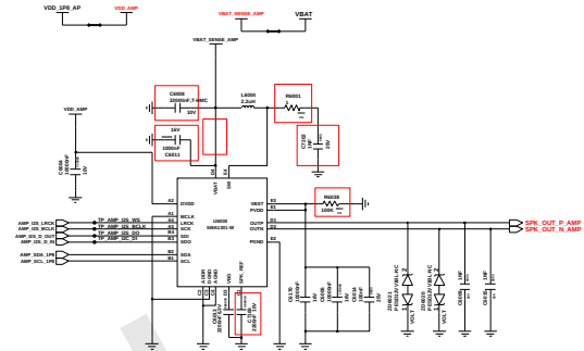
Audio amp
